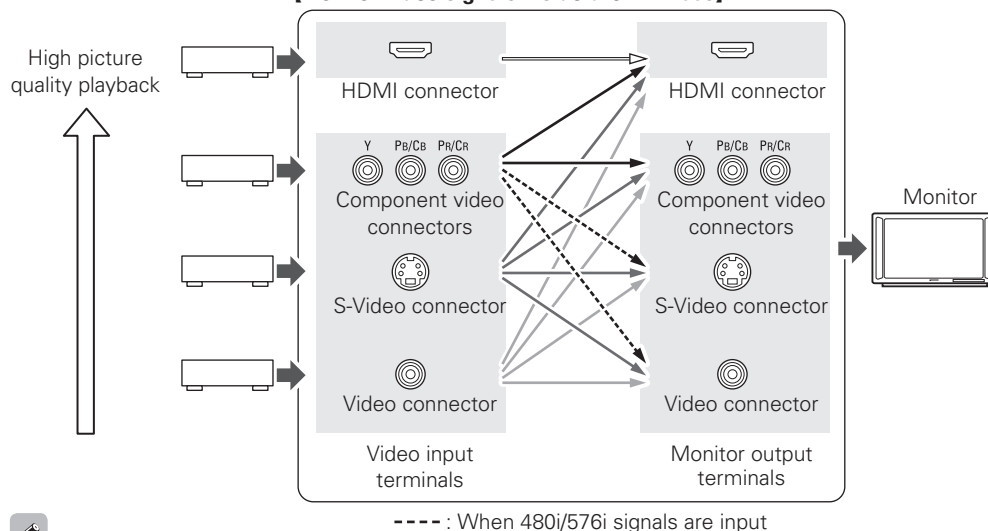
[Flow of video signals inside the AVR-889]
