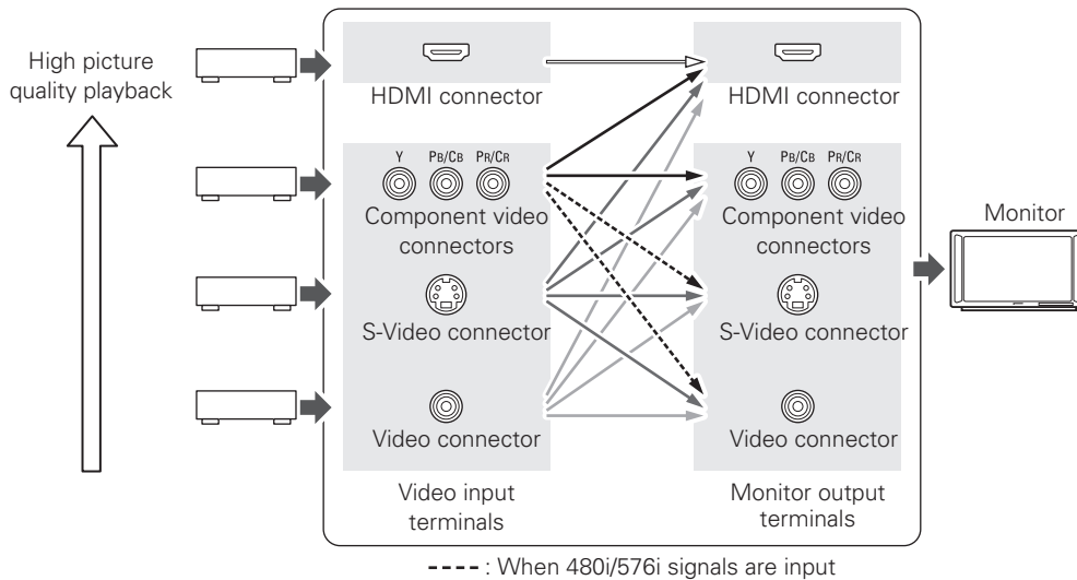
[Flow of video signals inside the AVR-1909]
