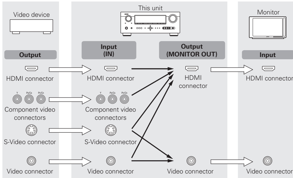
[Flow of video signals for MAIN ZONE]
