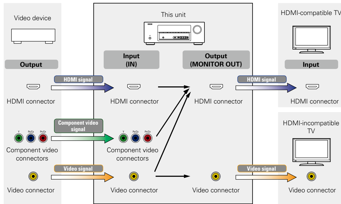
[Flow of video signals for MAIN ZONE]
