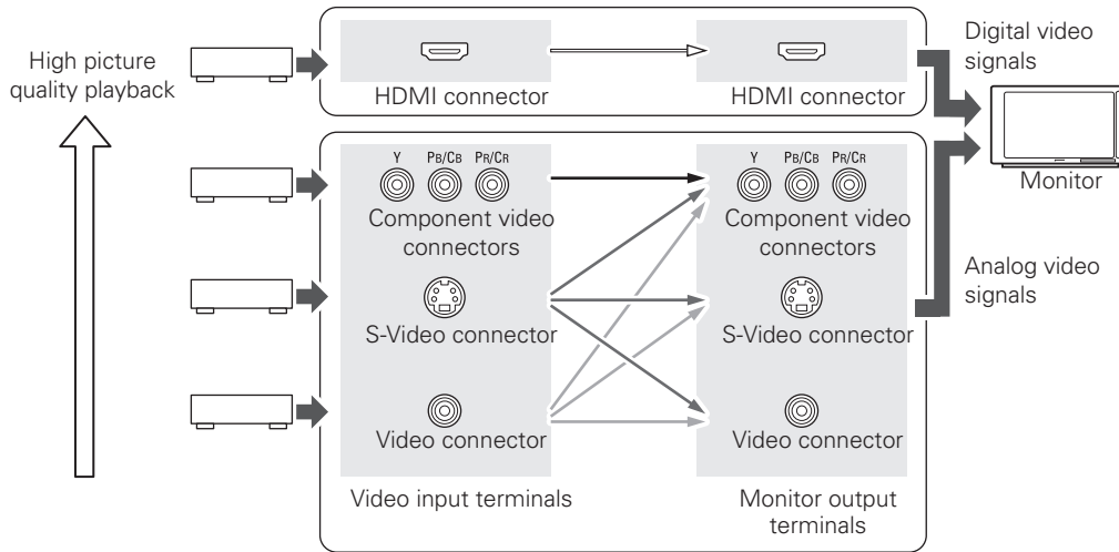
[Flow of video signals inside the AVR-1709]
